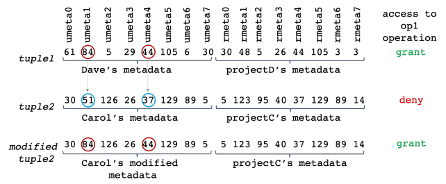
Figure 13: Applying Integrated Gradients to Grant Access.
